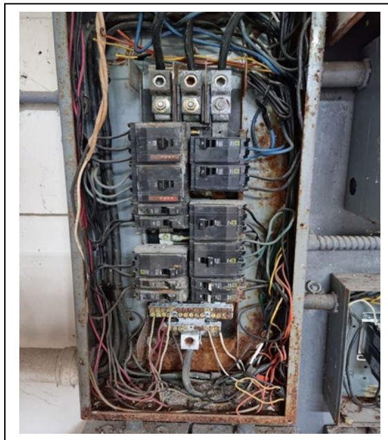
Photo of 30 circuit electrical panel which is to be replaced
